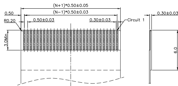
RECOMMENDED FPC/FFC DIMENSION
