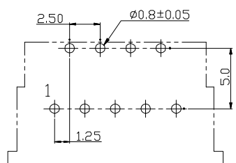
RECOMMEND PCB LAYOUT COMPONENT SIDE
