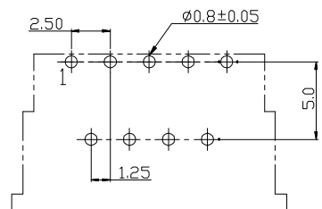
RECOMMEND PCB LAYOUT COMPONENT SIDE
