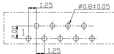
RECOMMEND PCB LAYOUT COMPONENT SIDE
