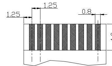
FFC/FPC DIMENSION THICKNESS 0.3±0.05mm
