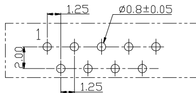
RECOMMEND PCB LAYOUT COMPONENT SIDE
